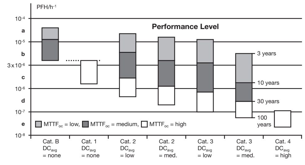
Relationship between categories DC, MTTF D and PL
